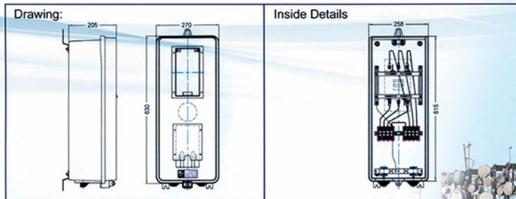
AF 400 (Standard type with single Breaker & Meter Mounting system)
